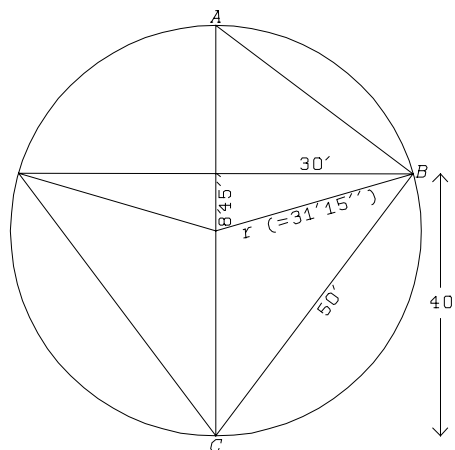
Figure 6. Redrawing of the triangle with circumscribed circle from TMS I
