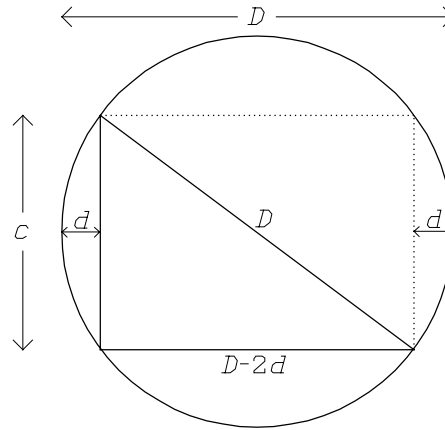
Figure 3. The circle of BM 85194 rev. I 33–43, with chord and descent.
