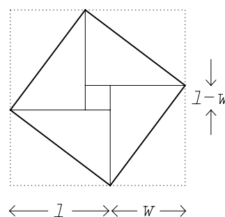
Figure 9, The initial steps of the procedure of Db 2 -146.
