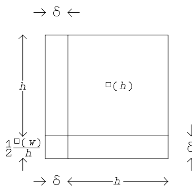
Figure 5. A possible geometrical procedure behind VAT 6598 #7.
