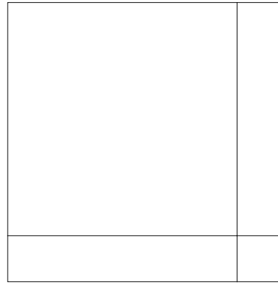
Figure 7. Diagram from which follows “proto- Elements II.7,” \square(R-r) = \square(R)-2\square(R,r)+\square(r) .
