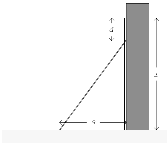
Figure 2. The pole standing and leaned against the wall.
