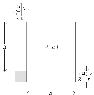
Figure 4. The probable geometrical reasoning behind VAT 6598 #6.
